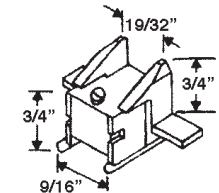
PART # 50605960 BOTTOM
