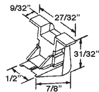
PART # 50605960 BOTTOM
