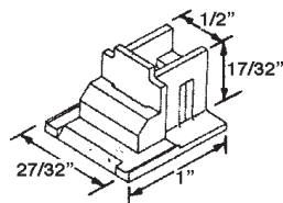
PART # 50605950 TOP
