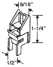
PART # 50605070 TOP
