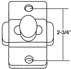
2-3/4" between screws, 2-hole PART # 50200240 (ZAMAK) PART # 50200242 (S/S)
