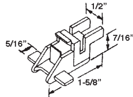
PART # 50605640 TOP
