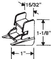
PART # 50605010 BOTTOM
