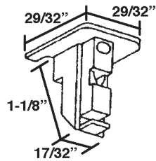
BOTTOM BRACKET PART # 50646010
