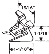
PART # 50605030 BOTTOM
