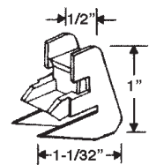
PART # 50605960 BOTTOM
