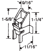
PART # 50605900 BOTTOM
