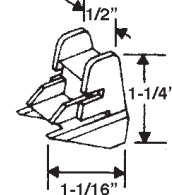
PART # 50605020 BOTTOM
