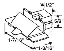
PART # 50605950 TOP
